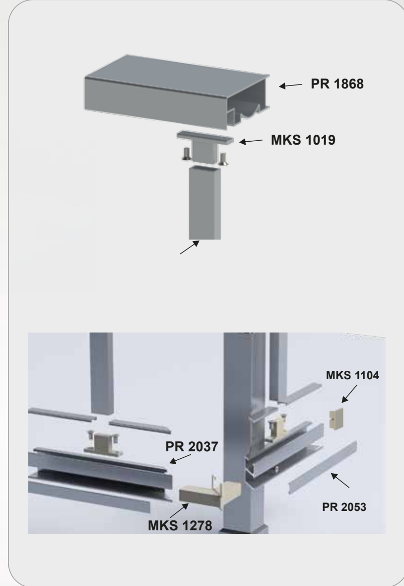
MODEL MKS 024-KESİT
